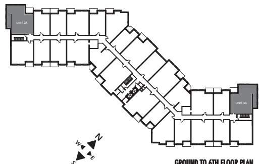
GROUND TO 6TH FLOOR PLAN
